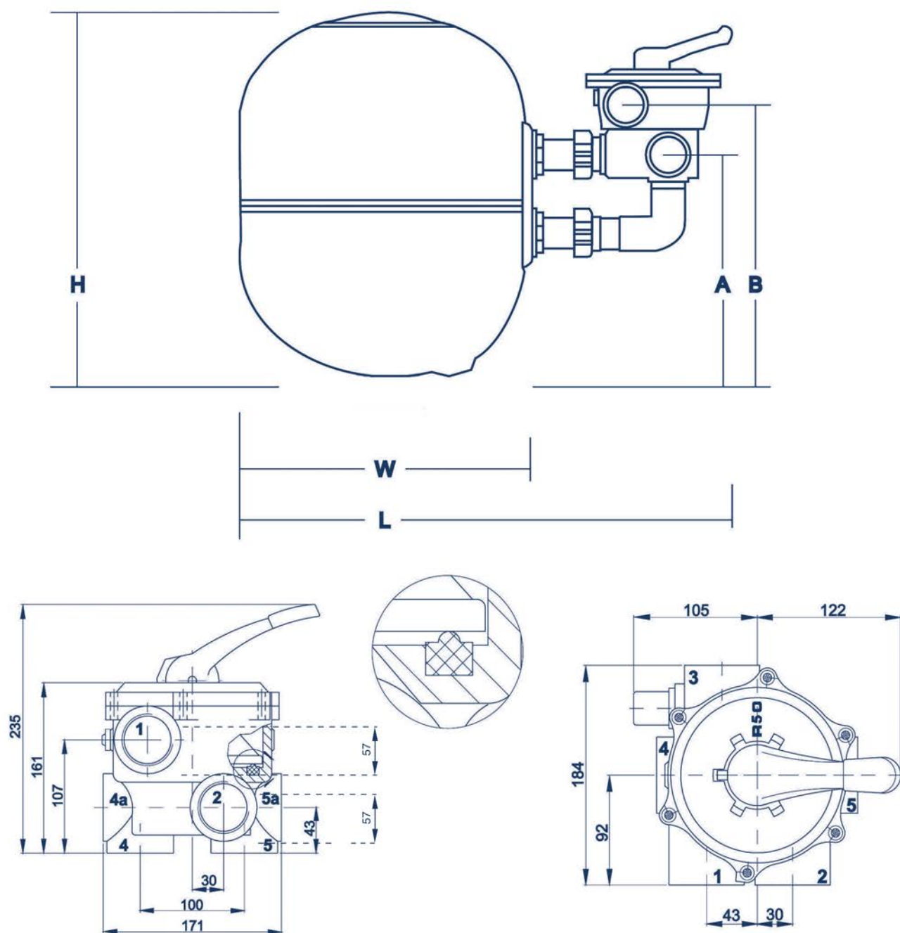
JUMBO dimension table (mm) / JUMBO-afmetingstabel (mm)
