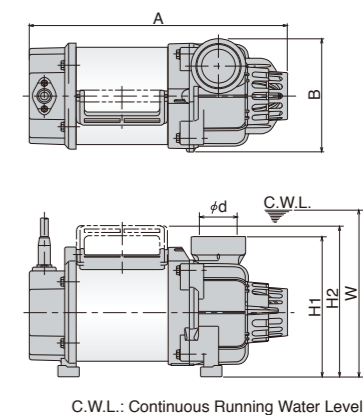
C.W.L.: Continuous Running Water Level
