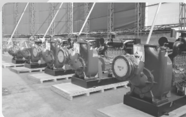
Skid Mounted
